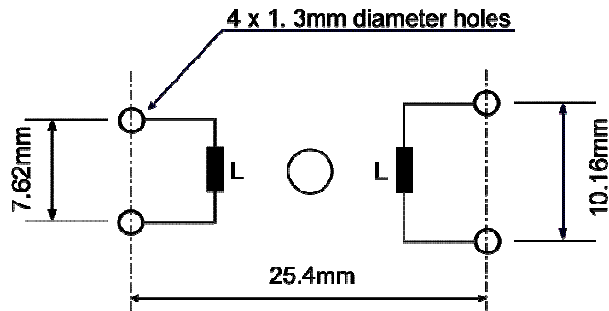
Mounting detail - top (component side) view
